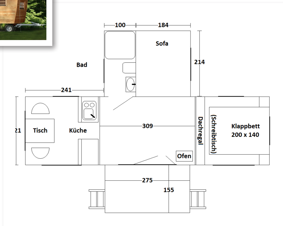
Grundriss Wohlwagen Basic. Innenmaße in cm.
